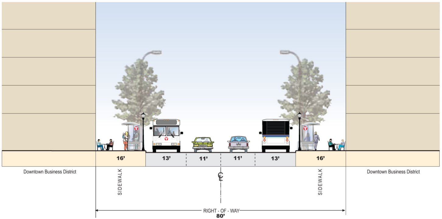
Alternate 1: No Parking, No Turn Lane
